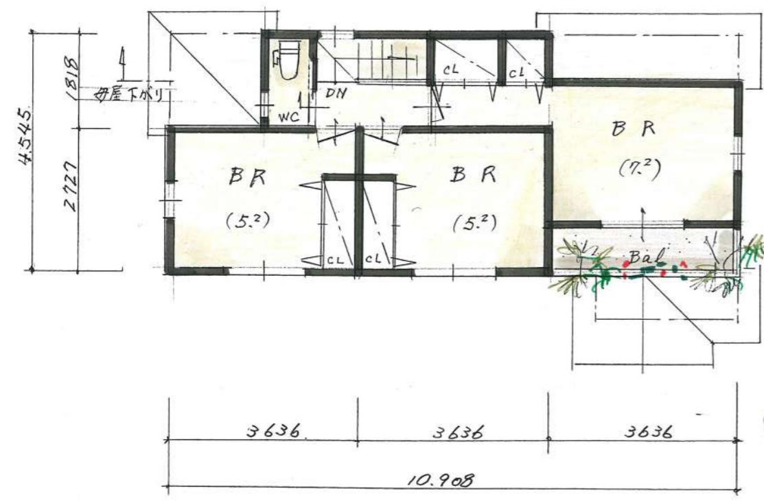
2F PLAN
